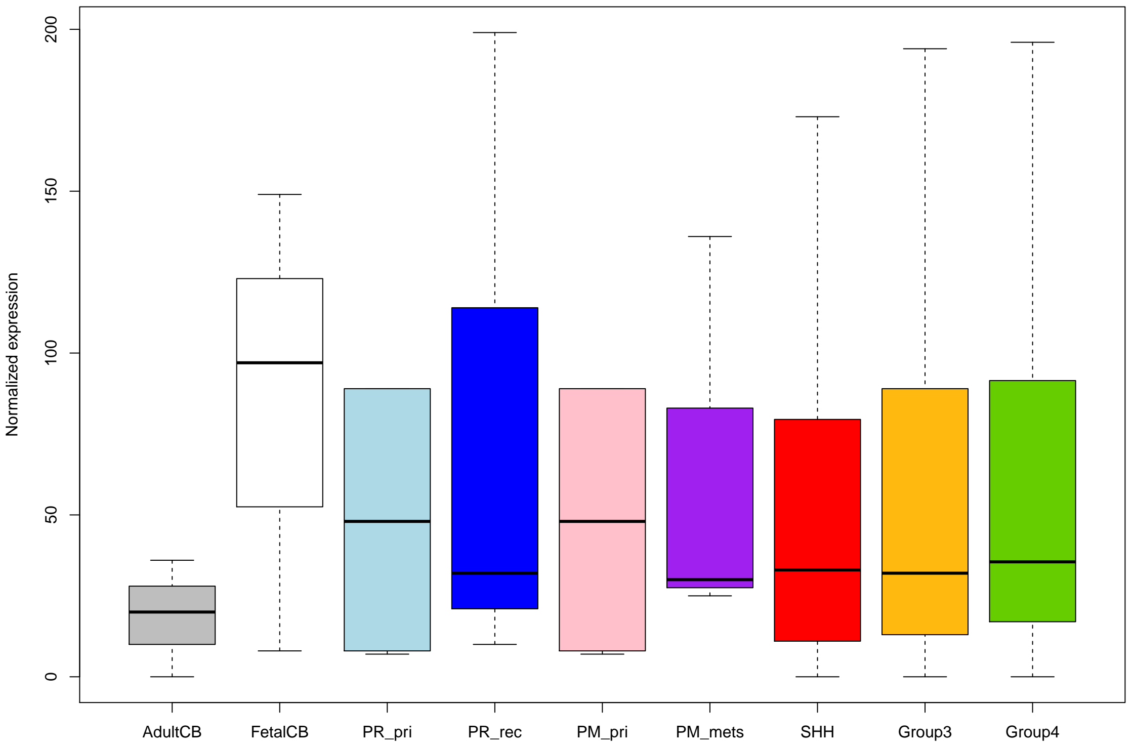
ENSG00000227921_AL353791.1_+ expression (no outliers)
