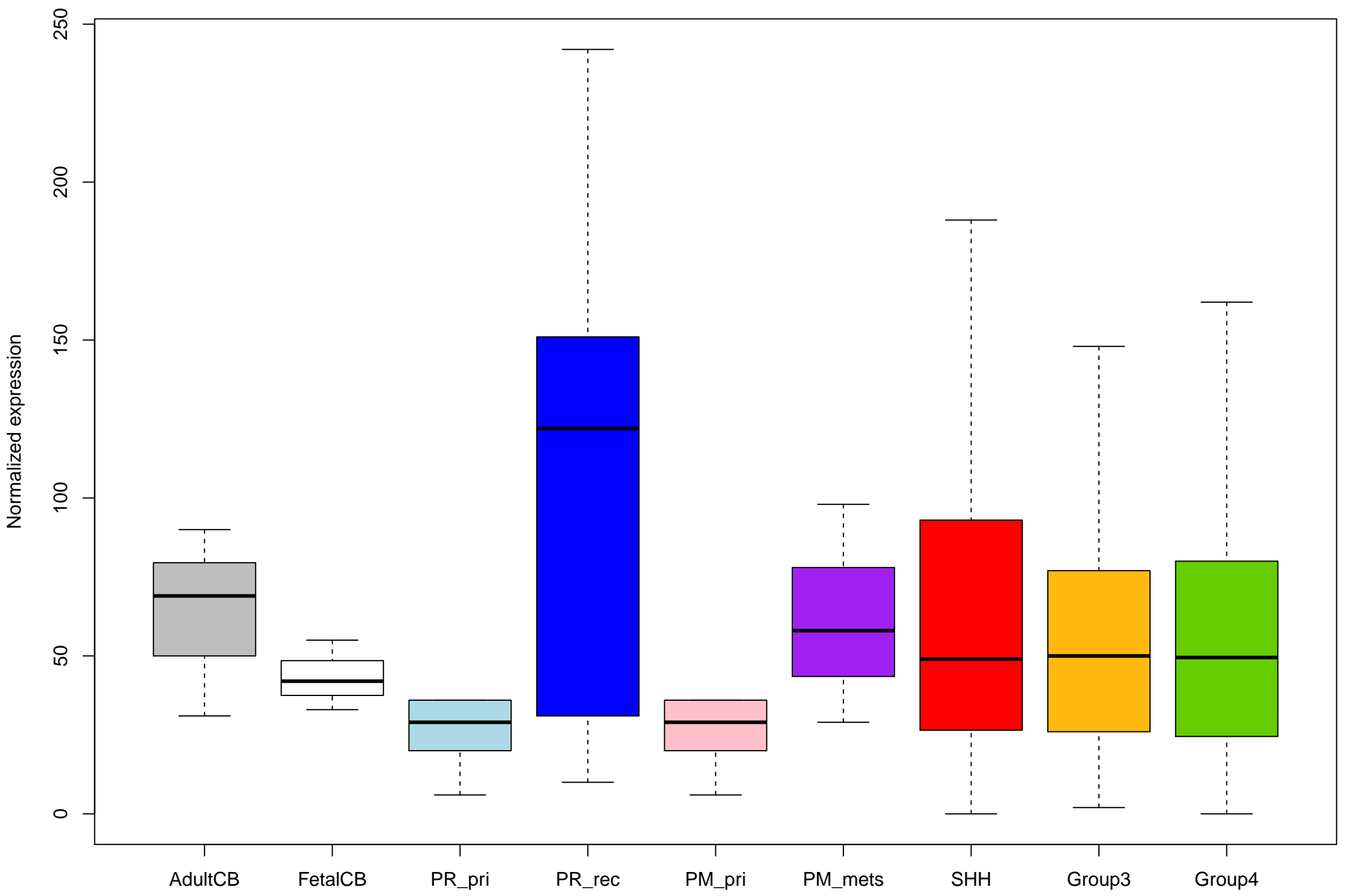
ENSG00000213413_PVRIG_+ expression (no outliers)
