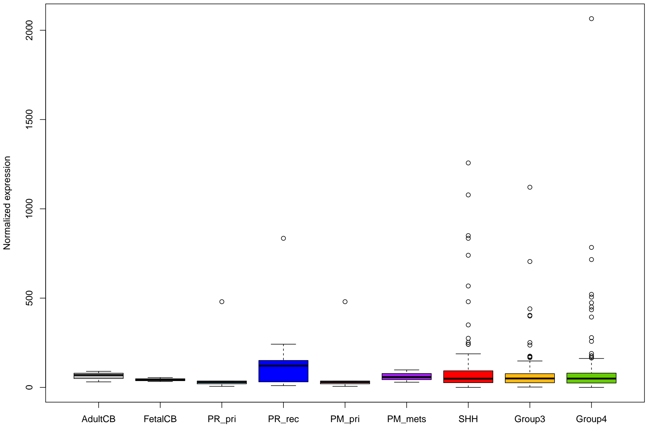
ENSG00000213413_PVRIG_+ expression (with outliers)
