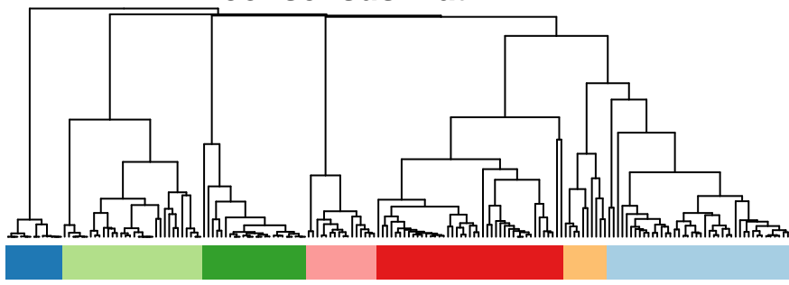
consensus matrix k=7
