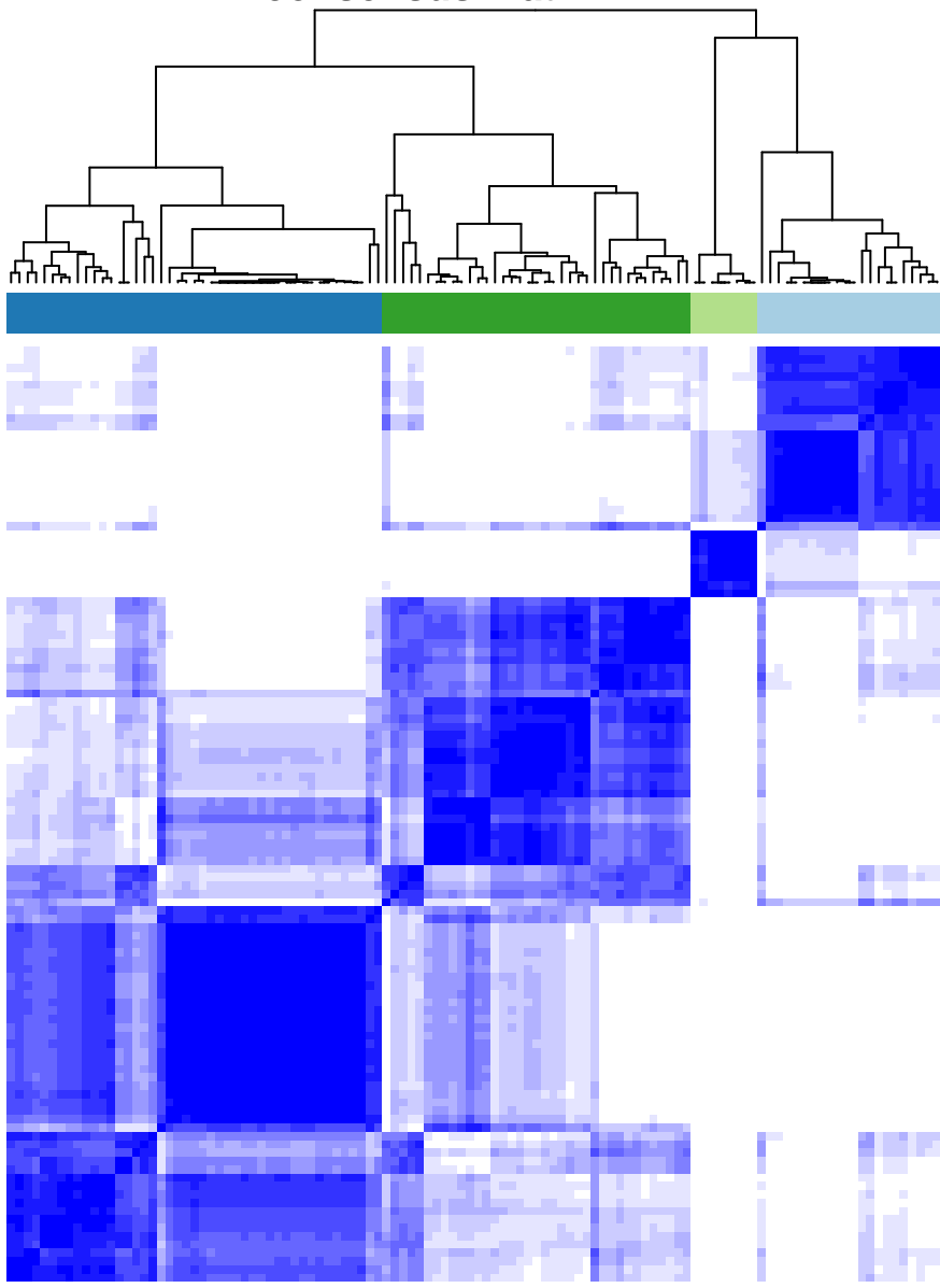
consensus matrix k=4
