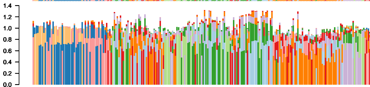
item-consensus k=9
