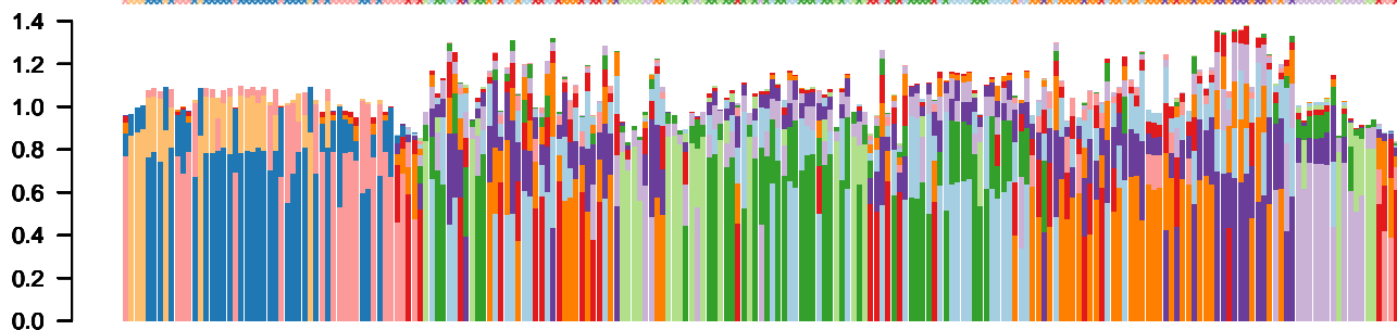
item-consensus k=10
