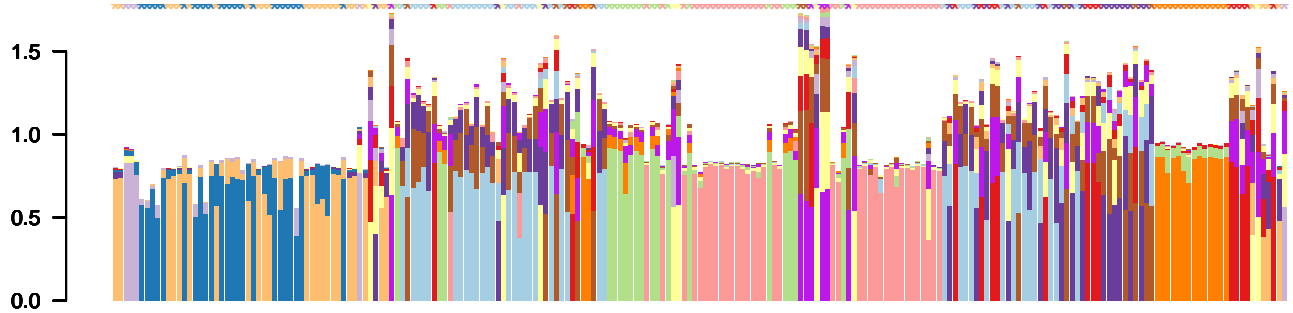
item-consensus k=12
