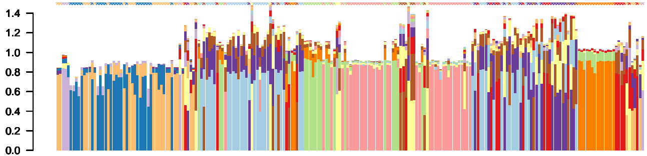
item-consensus k=11
